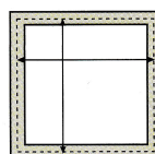
Borrowed Lite Width = Rabbet to Rabbet + 1 1/4" Height = Rabbet to Rabbet + 1 1/4" Note: Actual glass size is smaller. Always measure frame before ordering glass
