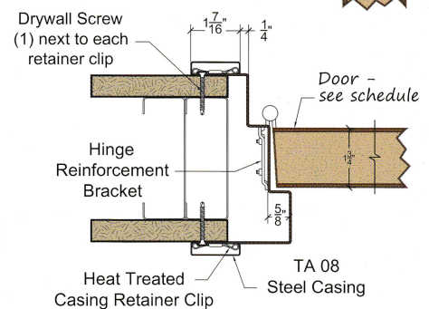
Upright-Double Egress
