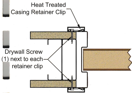
Inverted Stop Pocket Jamb
