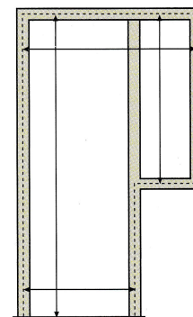
Door and Partial Sidelite UPPER: Nominal Door Width + Sidelite + 2" for each Mullion + 1 1/4" LOWER: Nominal Door Width + 1 1/4" Jamb Height + 1" Sidelite Height: Rabbet to Rabbet + 1 1/4"
