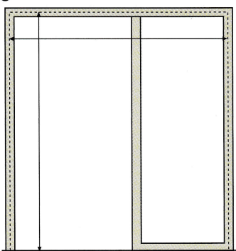
Door with Sidelite Nominal Door Width + Sidelite + 2" for each Mullion + 1 1/4" Jamb Height + 1"
